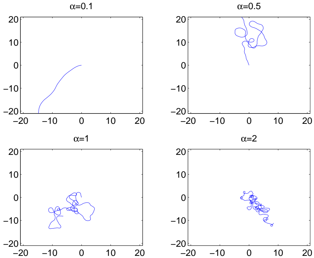
Figure 3: Four trajectories simulated with different value of \alpha : \alpha = 0.1 (top left), \alpha = 0.5 (top right), \alpha = 1 . (bottom left) and \alpha = 2 . (bottom right). The simulation is run during 120 time units with a time step dt = 0.05 time unit
