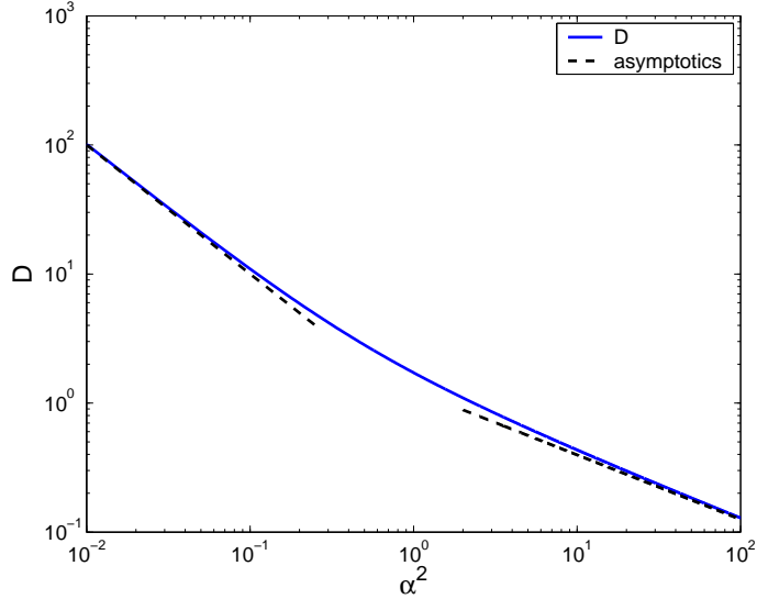
Figure 2: Scaled diffusion coefficient \mathcal{D} as a function of \alpha^2 in log-log scale (solid line). Asymptotic behavior of \mathcal{D} as \alpha \rightarrow 0 or \alpha \rightarrow \infty (dashed lines): \mathcal{D} \sim \alpha^{-2} as \alpha \rightarrow 0 and \mathcal{D} \sim \sqrt{\frac{\pi}{2}} \alpha^{-1} as \alpha \rightarrow \infty .
