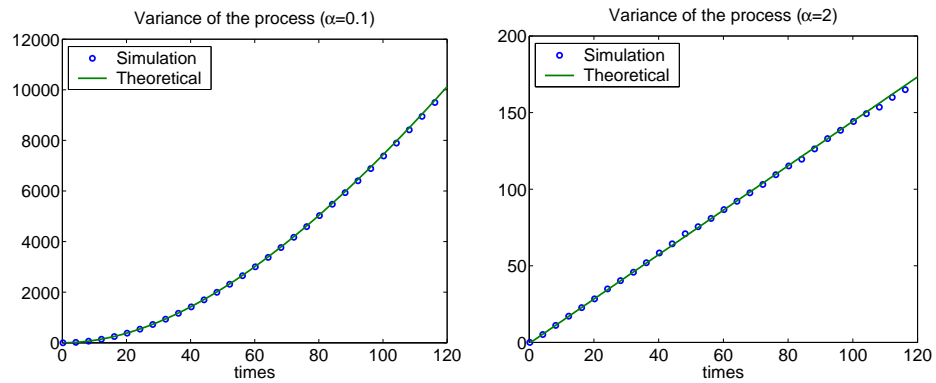
Figure 4: Variance of the process \vec{x}(t) : comparison between the numerical simulation (points) and the theoretical prediction (solid line) for two values of \alpha : \alpha = 0.1 (left) and \alpha = 2 (right).
