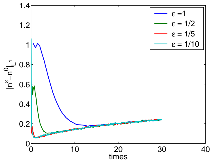
Figure 6: L^1 norm of the difference between n^\epsilon(t) = \int f^\epsilon(t, \cdot, \theta, \kappa) d\theta d\kappa and its asymptotic limit n^0(t) as a function of time t , with \alpha = 1 and N = 10^4 simulation particles.
