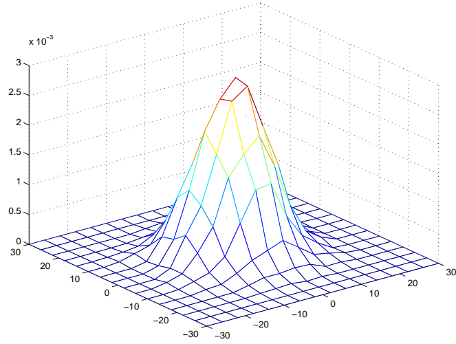
Figure 5: The spatial distribution n for \alpha = 2 at time T = 30 time units.
